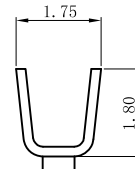
SEC: C-C
